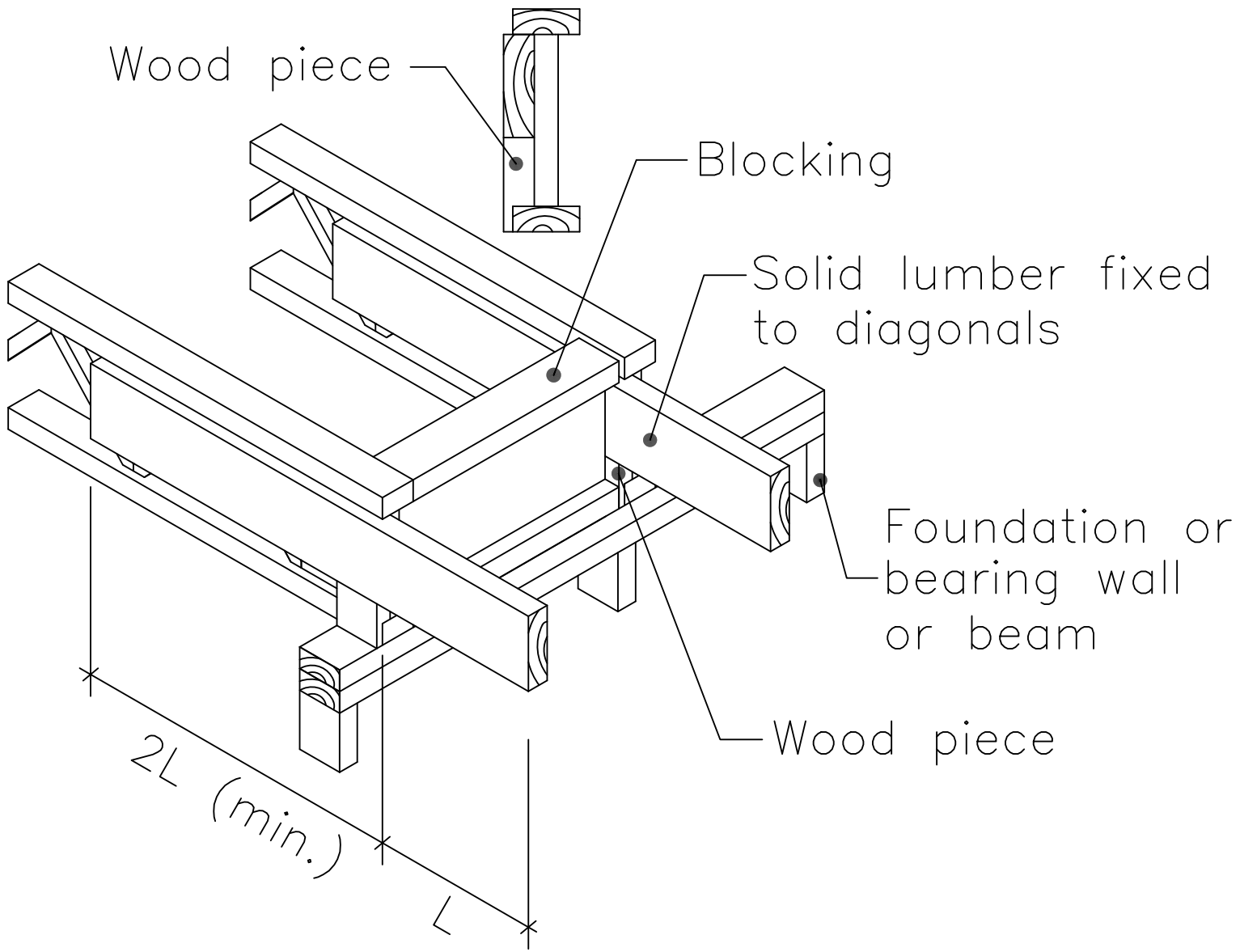
CANTILEVERED BALCONY
